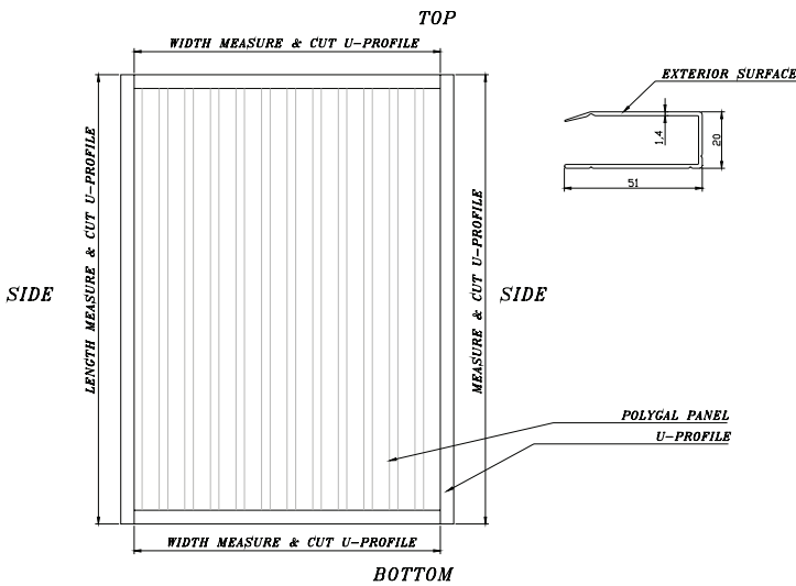
Typical Sheet Layout
