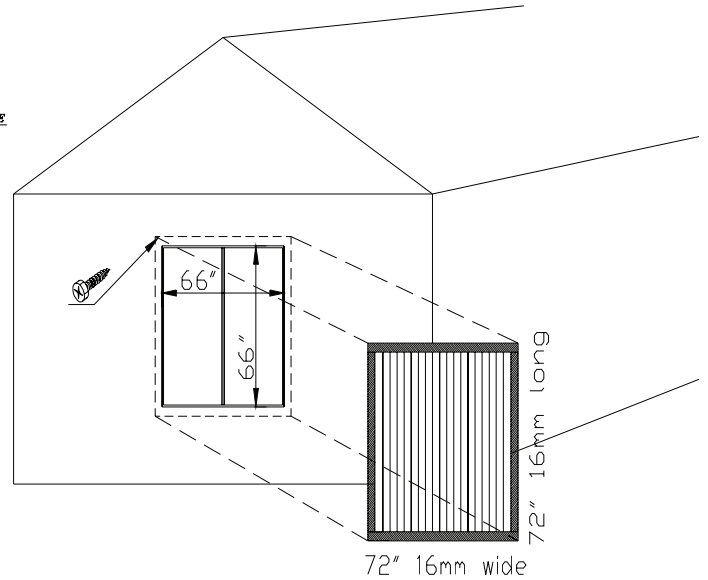
Typical Sheet Placement
