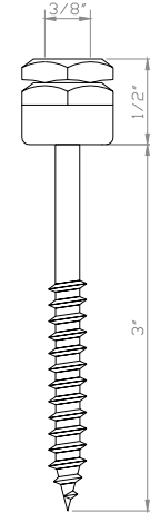
1-1/2" SAMMY for 3/8" Rod CST 20 for Concrete 3" SAMMY for 3/8" Rod GST 30 for Wood
