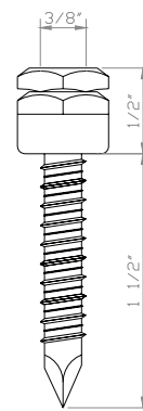
1-1/2" SAMMY for 3/8" Rod CST 20 for Concrete 3" SAMMY for 3/8" Rod GST 30 for Wood
