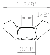
CF 3/8" - 16 Wing Nut
